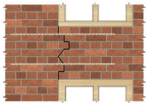
Crack stitching
