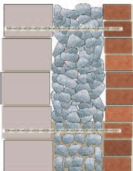
Stabilising bulging rubble-filled wall
